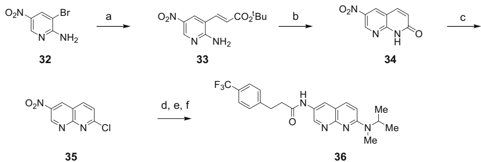
Scheme 3. Reagents and conditions: (a) tert -butyl acrylate, Pd(OAc) 2 , ( o -tol) 3 P, Et 3 N/DMF, 130 °C; (b) 5 N aq HCl, sealed tube, 130 °C; (c) POCl 3 , reflux; (d) N -methylisopropylamine, K 2 CO 3 , DMF, 80 °C; (e) H 2 , Pd-C, MeOH; (f) RCOCl, Et 3 N, CH 2 Cl 2 .
