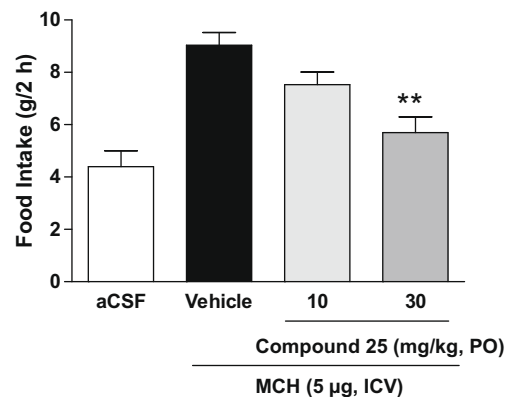
Figure 2. Effect of compound 25 on MCH-induced feeding response in SD rats. Values are the mean \pm SEM of 15–20 rats per group. ** P < 0.01 versus vehicle/MCH group.
