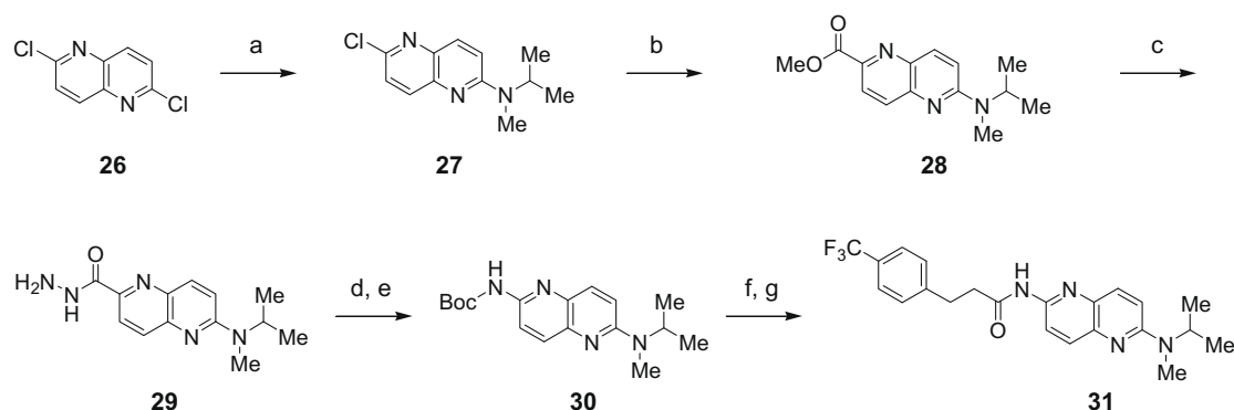
Scheme 2. Reagents and conditions: (a) N -methylisopropylamine (10 equiv), dioxane, sealed tube, 120 °C; (b) CO (140 psi), Pd(dppf)Cl 2 ·CH 2 Cl 2 , NaHCO 3 , MeOH/dioxane, 100 °C; (c) NH 2 NH 2 ·H 2 O, MeOH; (d) NaNO 2 , 1 N aq HCl, 0 °C; (e) tert -BuOH/dioxane, reflux; (f) CF 3 COOH; (g) RCOCl, pyridine, CHCl 3 .
