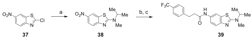
Scheme 4. Reagents and conditions: (a) N -methylisopropylamine (3 equiv), K 2 CO 3 , DMF, 80 °C; (b) H 2 , Pd-C, MeOH/THF; (c) RCOOH, 2-chloro-1,3-dimethylimidazolidinium chloride, pyridine, CHCl 3 .
