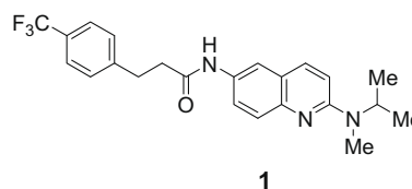
Figure 1. Aminoquinoline MCH1R antagonist.
