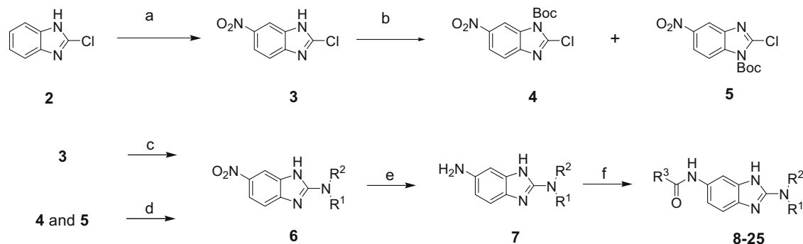
Scheme 1. Reagents and conditions: (a) 70% HNO 3 , H 2 SO 4 ; (b) Boc 2 O, DMAP, THF; (c) R 1 R 2 NH (8–50 equiv), neat or in dioxane, sealed tube, 130 °C; (d) R 1 R 2 NH or HCl salt (2.2–3.3 equiv), DIEA, dioxane or DMSO, 80–100 °C; (e) H 2 , Pd(OH) 2 -C, MeOH; (f) R 3 COOH, HATU, DIEA, CH 2 Cl 2 or R 3 COCl, Et 3 N, CH 2 Cl 2 .
